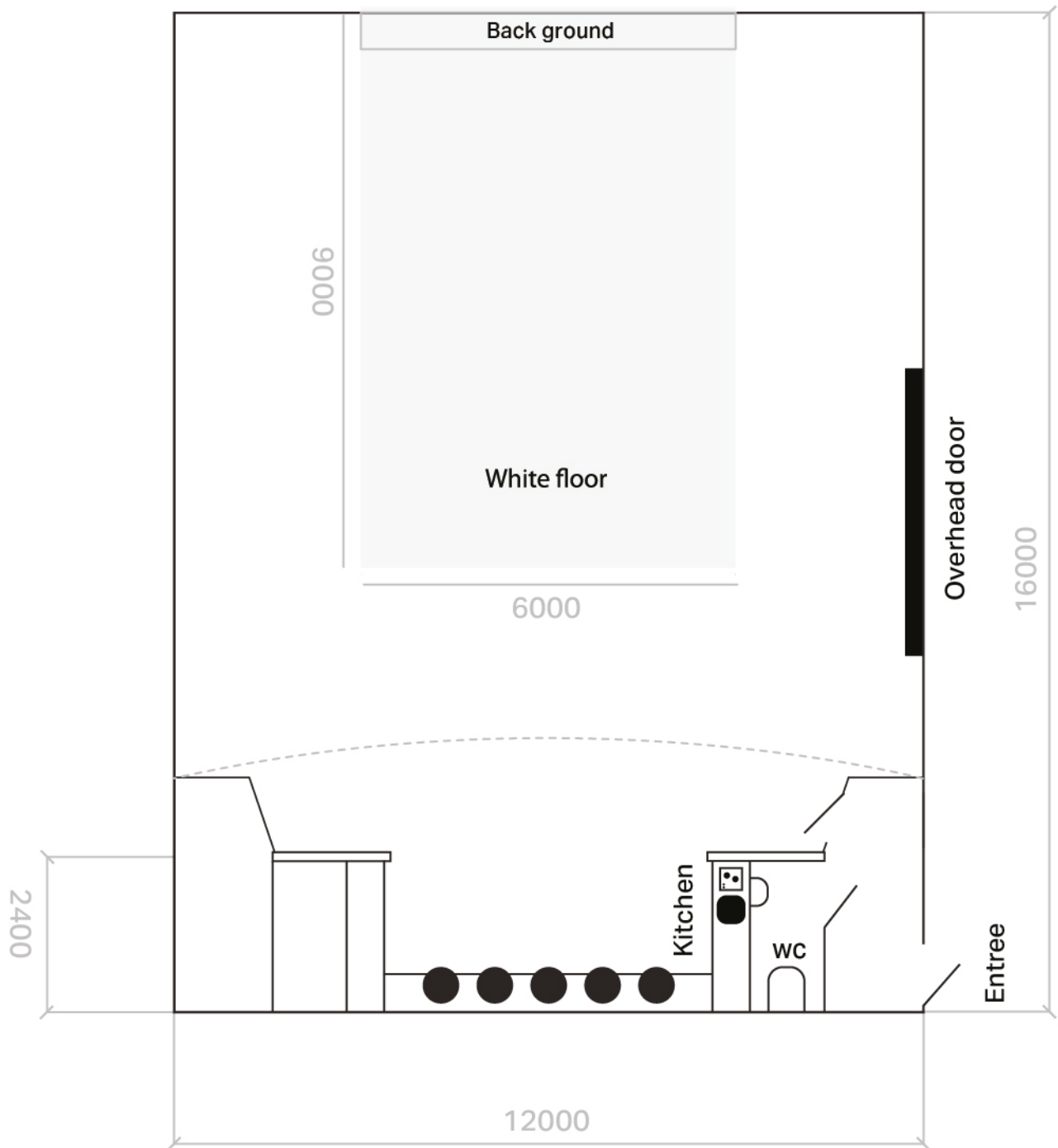
Ground Floor
